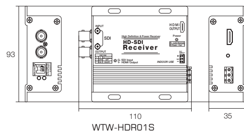
WTW-HDR01S
