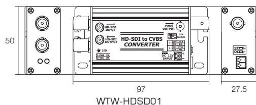
WTW-HDSD01
