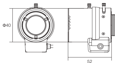
M13VG288IR
