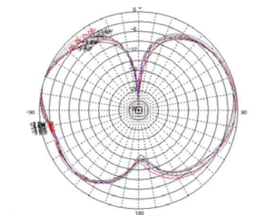
Vertical Pattern
