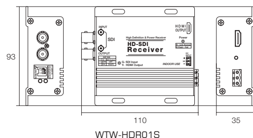
WTW-HDR01S
