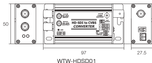
WTW-HDSD01
