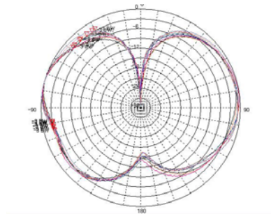
Vertical Pattern
