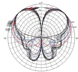
Vertical Pattern
